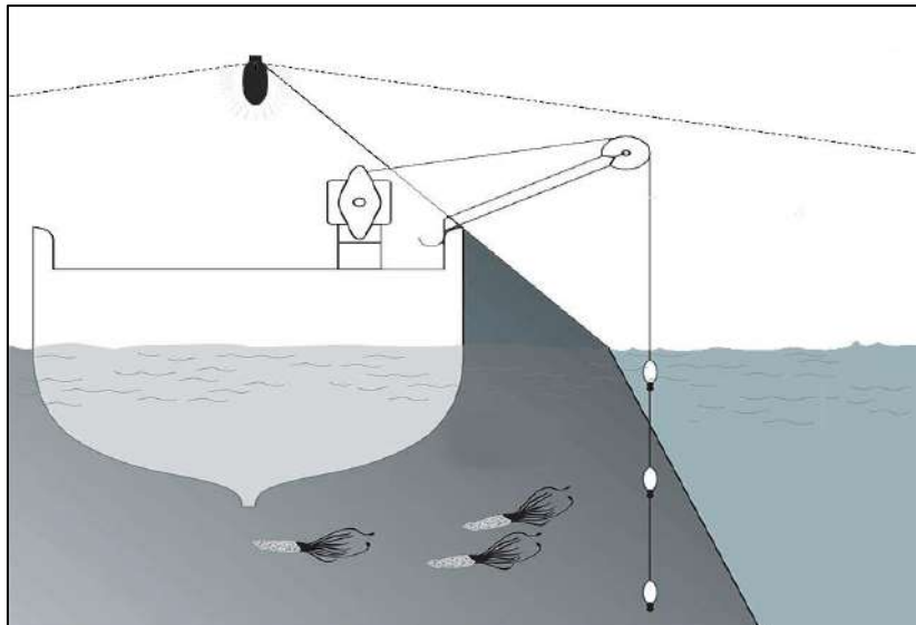
Gambar pancing cumi mekanis
